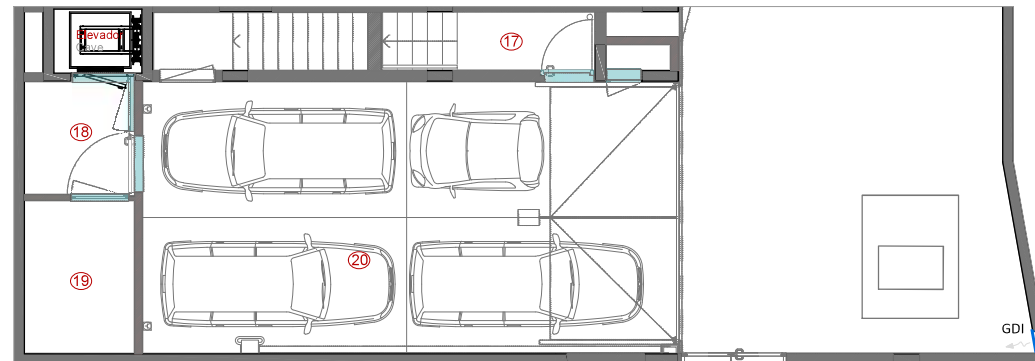
PISO CAVE
